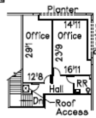
Mezzanine Office Plan
